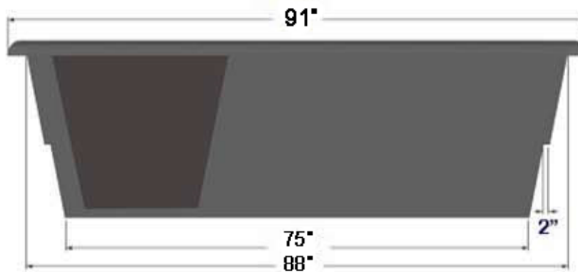
Base Dimensions
